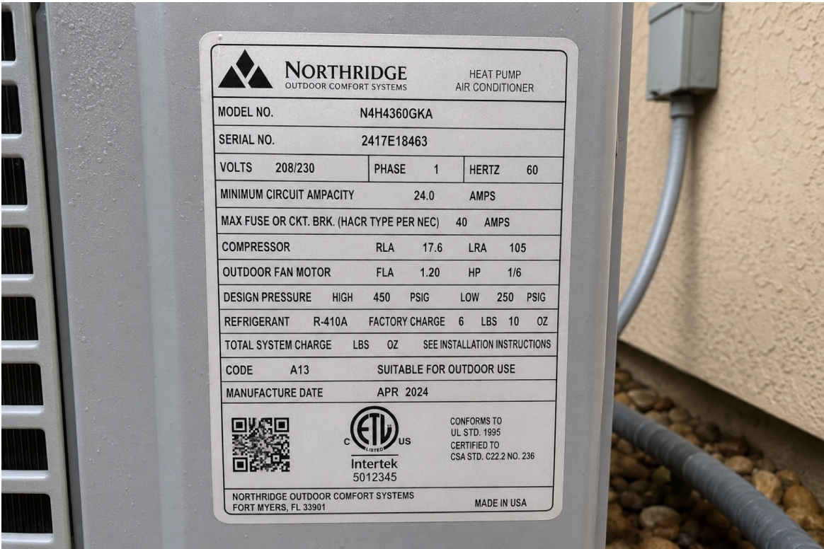
HVAC — photo 2
